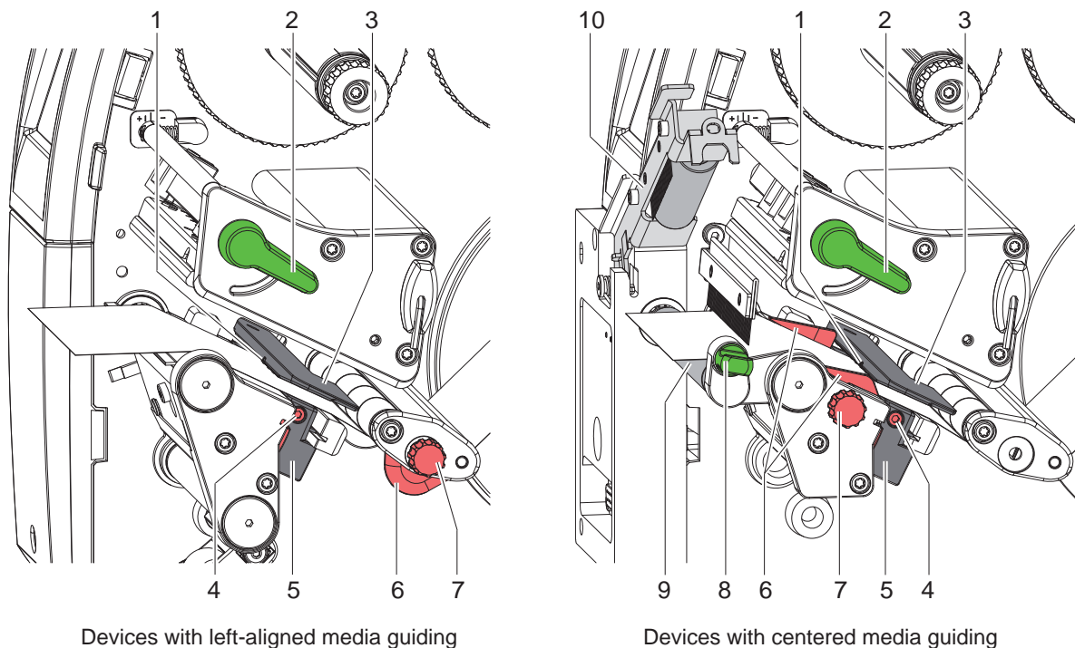
Figure 13 Inserting the media into the printhead
