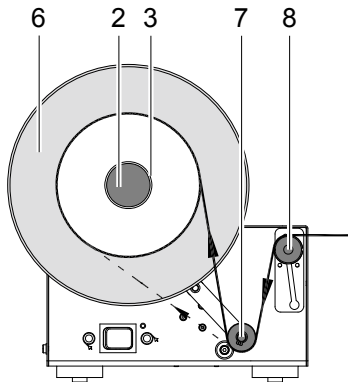
Figure 9 Rewinding onto 40 mm (1.6 in) cardboard core (drawing below without plate)
