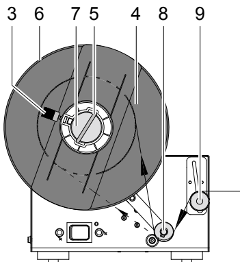
Figure 7 Direct rewinding
