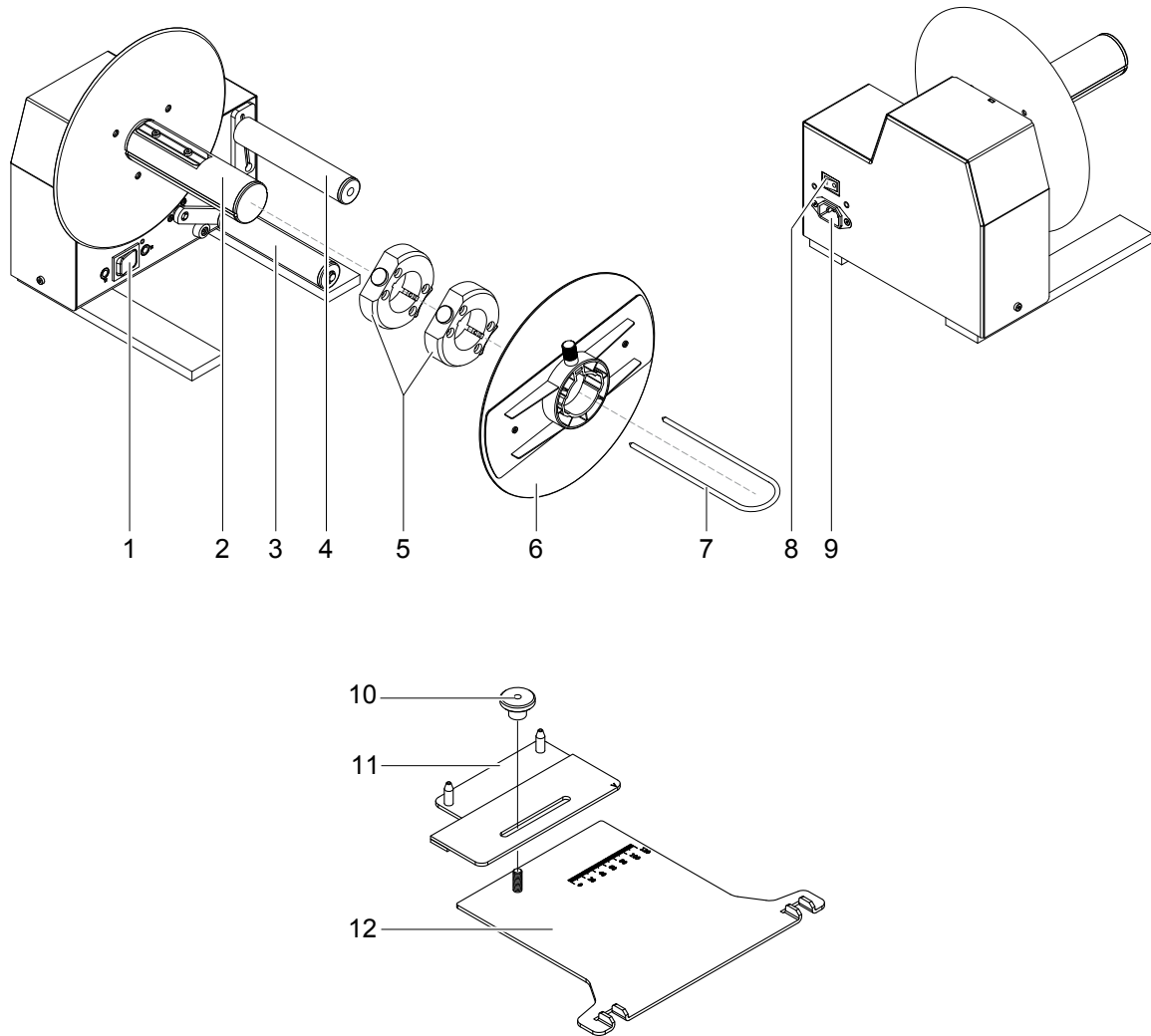
Figure 1 Device overview
